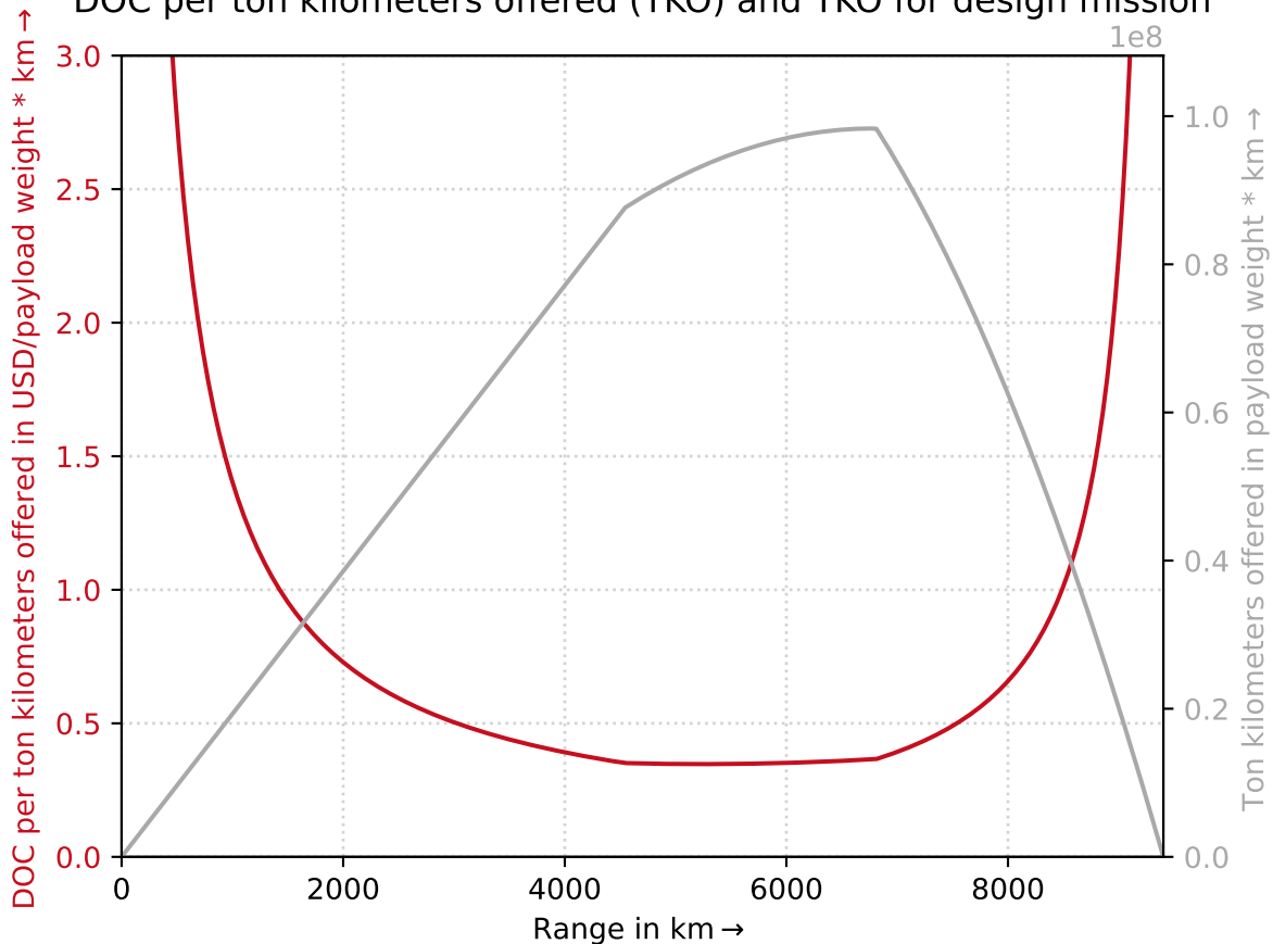
DOC per ton kilometers offered (TKO) and TKO for design mission
